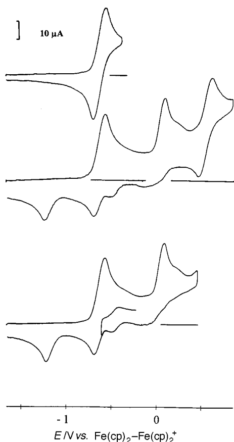
Fig. 1 Cyclic voltammety of [\text{Mo}_2(\text{cp})_2(\mu\text{-SMe})_3(\mu\text{-NH}_2)] 1 (ca. 2 mM) in thf- [\text{NBu}_4][\text{PF}_6] (vitreous carbon electrode, scan rate: 0.2 V s -1 )
