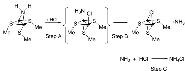
Scheme 3 ● = Mo(cp)
