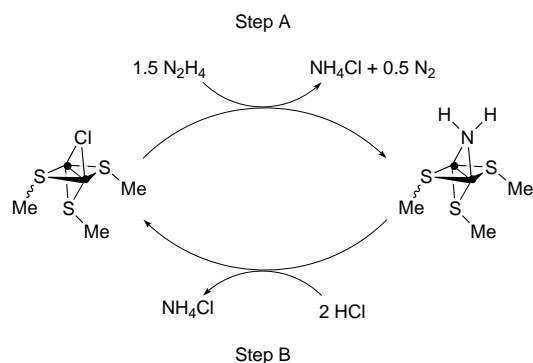
Scheme 4 ● = Mo(cp)
