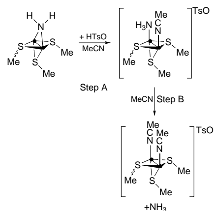
Scheme 5 ● = Mo(cp)
