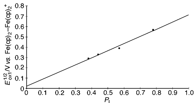
Fig. 6 Plot of E_{\text{ox1}}^{1/2} of the protonated complexes [\text{Mo}_2(\text{cp})_2(\mu\text{-SMe})_3(\text{NH}_3)(\text{L or X}^-)]^+ vs. the ligand constant P_L 16 (L or \text{X}^- = \text{xyI NC} , \text{Bu}^i\text{NC} , thf or \text{CF}_3\text{CO}_2^- )
