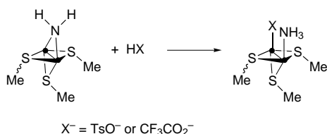
Scheme 2 ● = Mo(cp)
