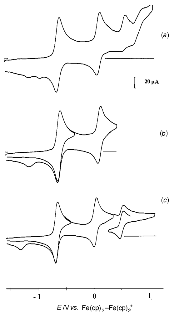
Fig. 2 Cyclic voltammety of [\text{Mo}_2(\text{cp})_2(\mu\text{-SMe})_3(\mu\text{-NH}_2)] 1 (2.2 mM) in MeCN- [\text{NBu}_4][\text{PF}_6] at room temperature (a,b) and at -46 °C (c) (vitreous carbon electrode, scan rate: 0.2 V s -1 )
